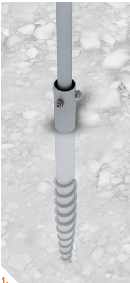
1. Attaching the legs to the ground screw allows the height of the structure to be adjusted
